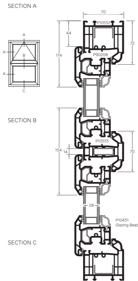
Storm70 72mm Outer Frame Large
