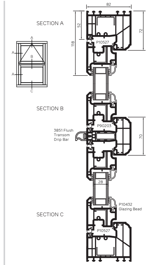
Flush82 72mm Outer Frame Large
