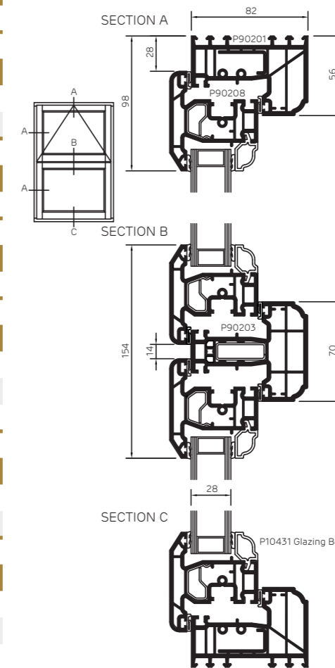
Storm82 56mm Outer Frame Slim
