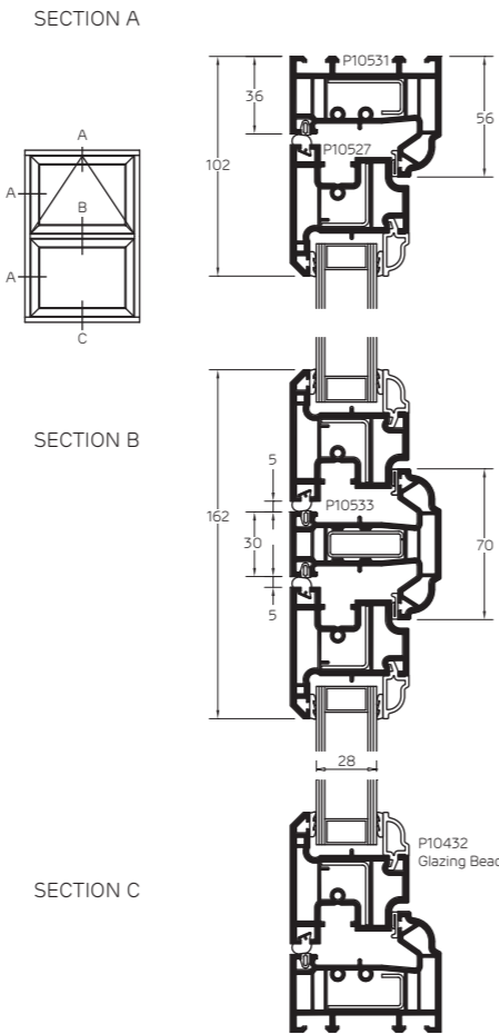
Flush70 56mm Outer Frame Slim
