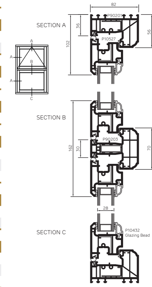
Flush82 56mm Outer Frame Slim
